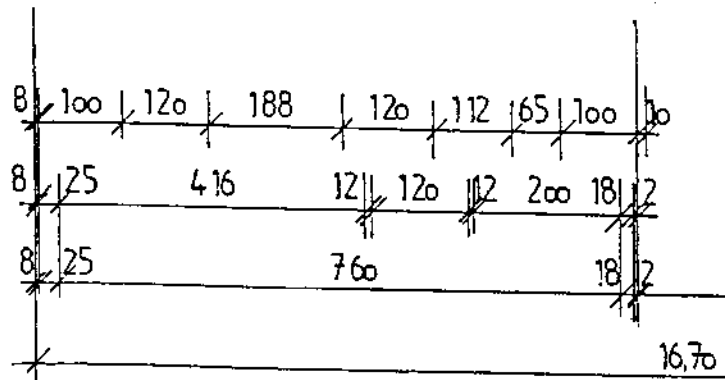
TOP ⑤ WF: 35,25□
